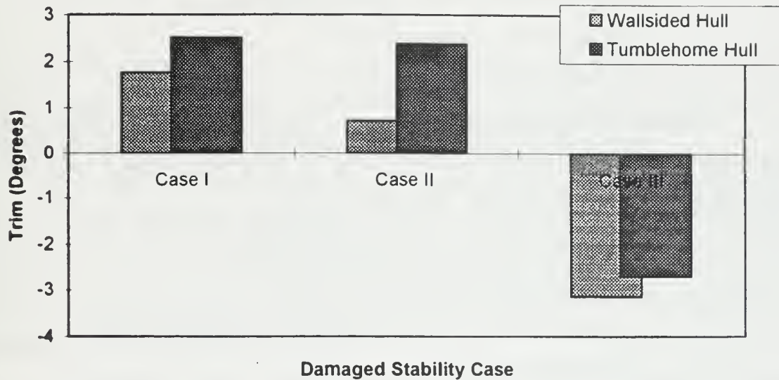
Figure 15. Trim Analysis
